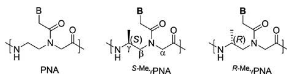
Chart 1. Chemical Structures of PNA and \gamma PNA Units
