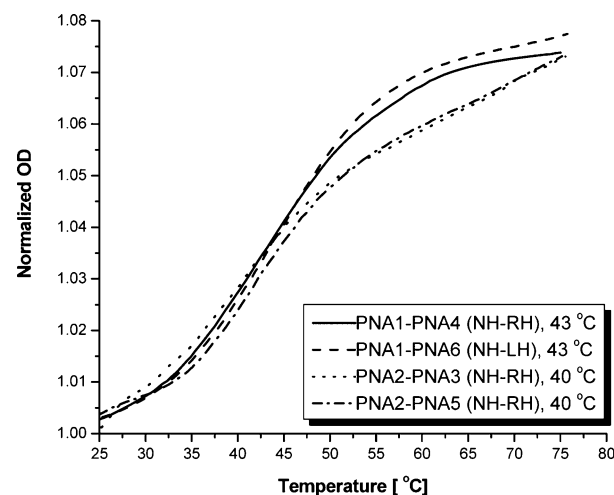
Figure 6. UV-melting profiles of PNA– \gamma PNA heteroduplexes, with the latter containing RH and LH helical motifs at 5 \mu M strand concentration each.
