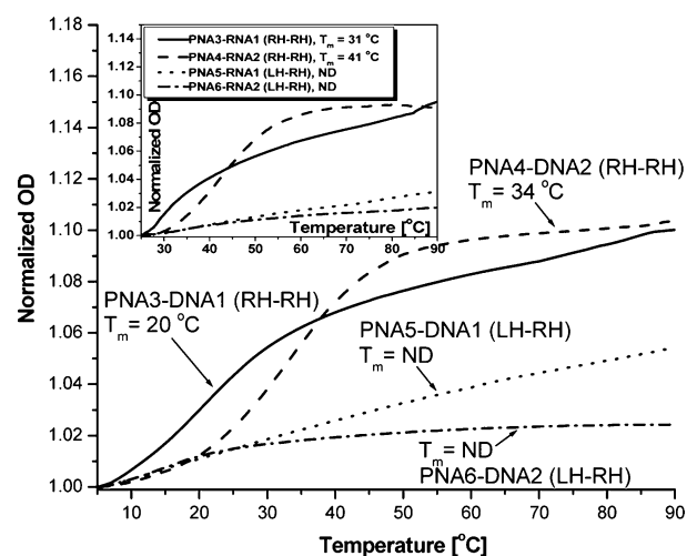
Figure 5. UV-melting profiles of \gamma PNA–DNA pairs with matched (RH–RH) and mismatched (LH–RH) helical sense at 5 \mu M strand concentration each. Inset: melting curves of \gamma PNA–RNA pairs. DNA1:5′-GTTGG-3′, DNA2:5′-CCAAC-3′, RNA1:5′-GUUGG-3′, RNA2:5′-CCAAC-3′.
